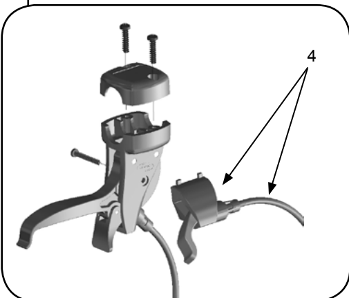
Combination Hand Activated Brake & Single Hand Activated Tilt “Green Trigger Tilt”
